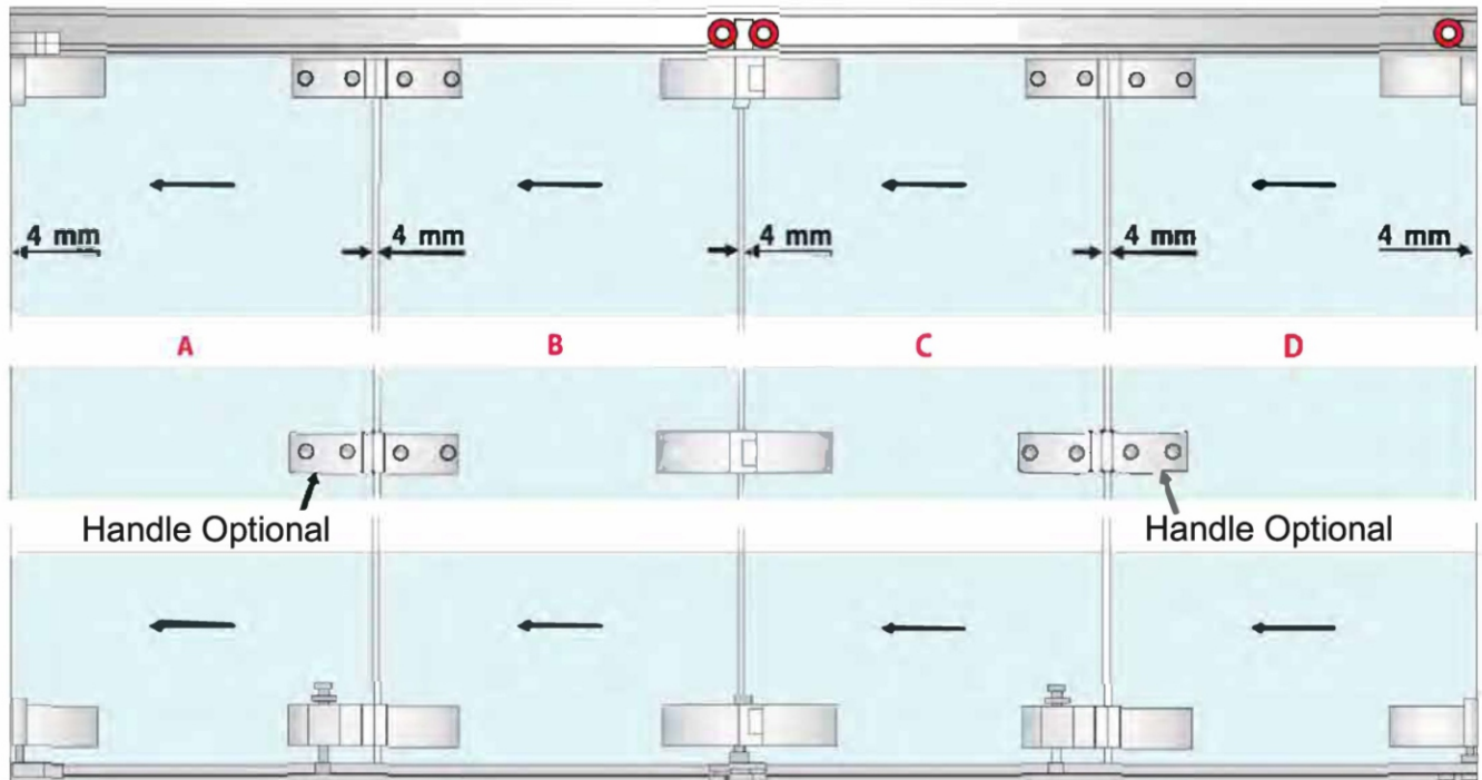
Glass Preparation for A, B & C
