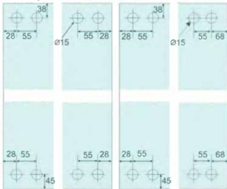
Glass Preparation for A, B & C
