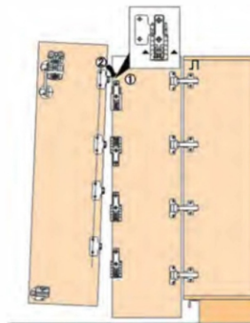
2. Hinge Connecting
