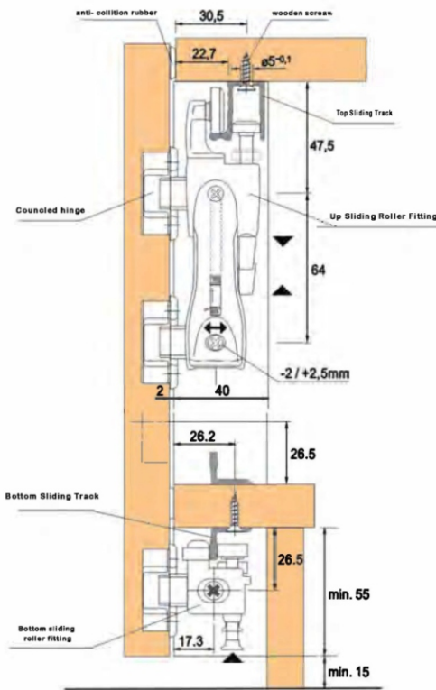
Folding Door Installation Sizes & Flight View
