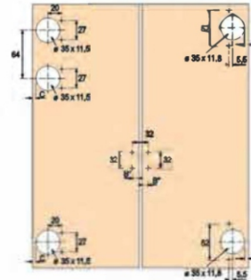
1. Hinge Hole Sizes And Situations
