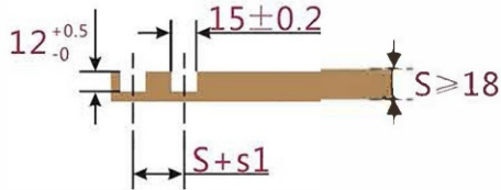
Slot dimension for aluminum rail
