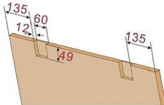
Runner installation
