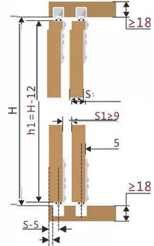
Wardrobe dimension
